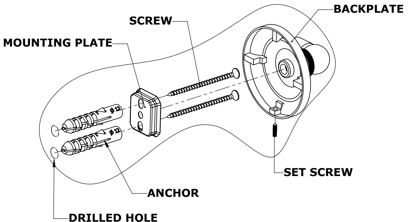
DETAIL O
